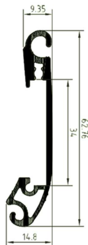
Lama autoblocante PS15 monopared 60668
